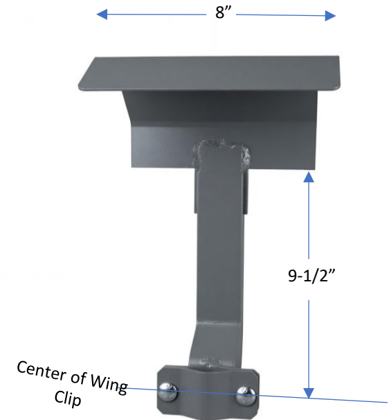
The Wing Clip measures at 2" X 4-1/4"
